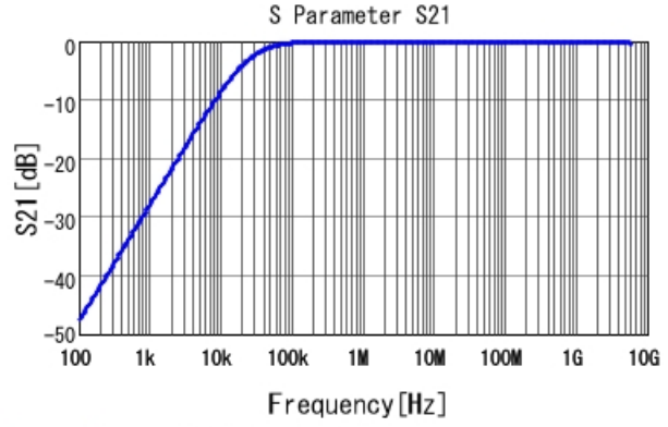
GRM155R61C683KA88 S21 DC0V, 25degC
