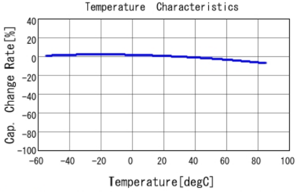
GRM155R61C683KA88 C-Temp. capchange, DC0.0V, AC1.C
