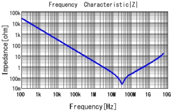
GRM155R61C683KA88 |Z| DCOV, 25degC
