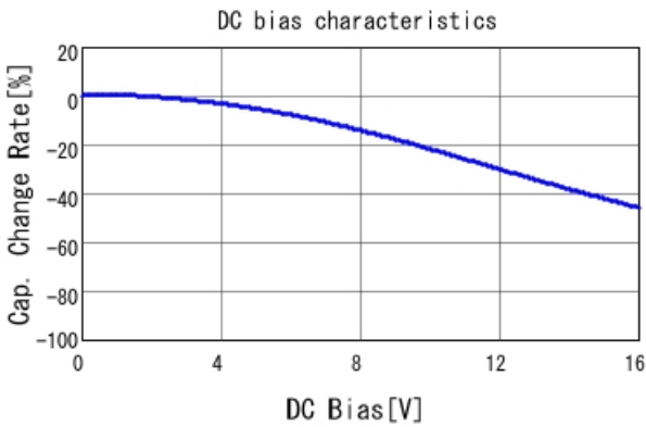
GRM155R61C683KA88 C-DC bias capchange, 25.0degC, A
