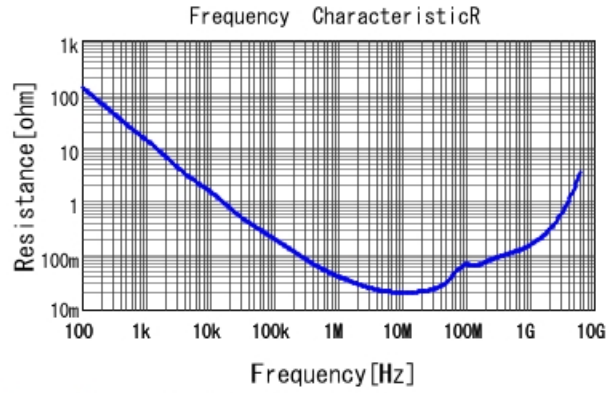
GRM155R61C683KA88 R DCOV, 25degC
