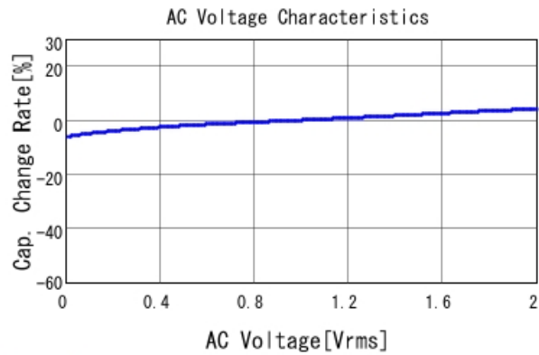
GRM155R61C683KA88 C-AC Voltage capchange, DCOV, 25
