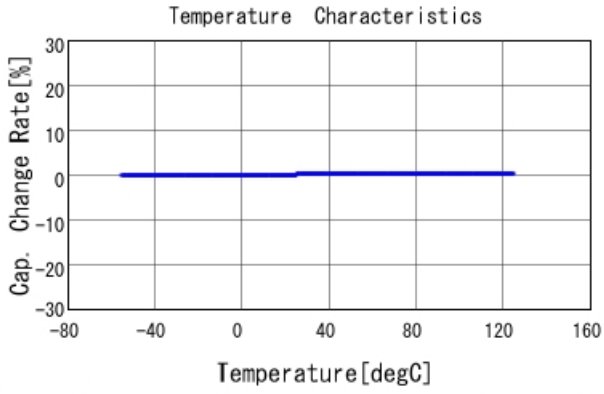
GJM1555C1H5R1CB01 C-Temp. capchange, DCOV, AC1Vrms
