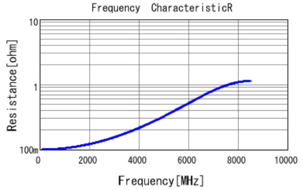
GJM1555C1H5R1CB01 R DCOV, 25degC
