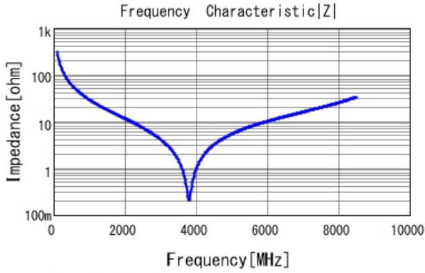
GJM1555C1H5R1CB01 |Z| DCOV, 25degC
