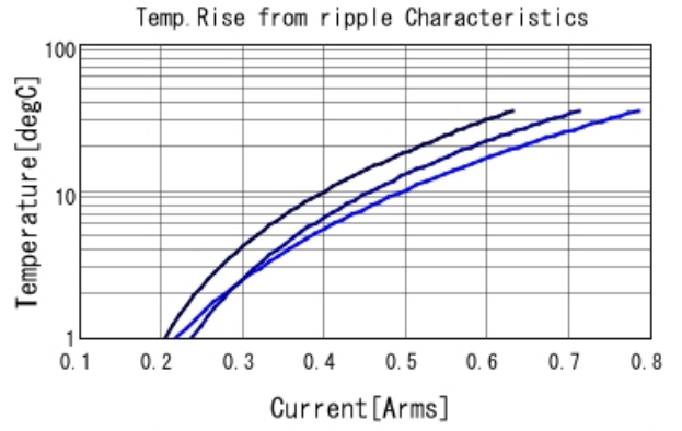
GJM1555C1H5R1CB01 Temp. rise — 1GHz — 2GHz
