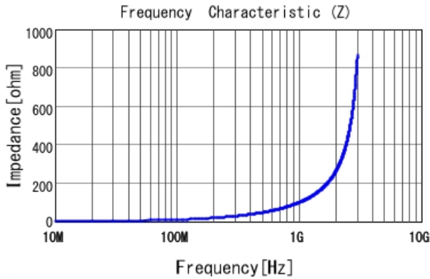
LQP03TN15NJZ2 |Z|
