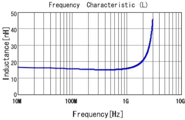
LQP03TN15NJZ2 L
