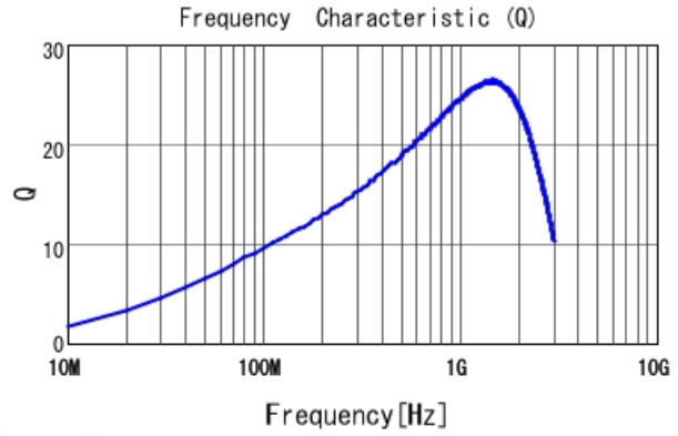
LQP03TN15NJZ2 Q
