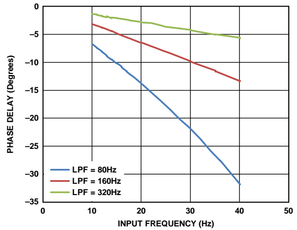
Figure 19. Low-Pass Filter Phase Delay
