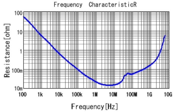
GCM188R71E154KA37 R DCOV, 25degC
