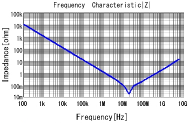
GCM188R71E154KA37 |Z| DCOV, 25degC
