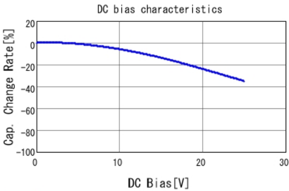
GCM188R71E154KA37 C-DC bias capchange, 25.0degC, A
