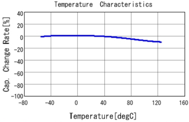
GCM188R71E154KA37 C-Temp. capchange, DC0.0V, AC1.C
