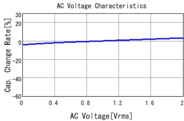
GCM188R71E154KA37 C-AC Voltage capchange, DCOV, 25
