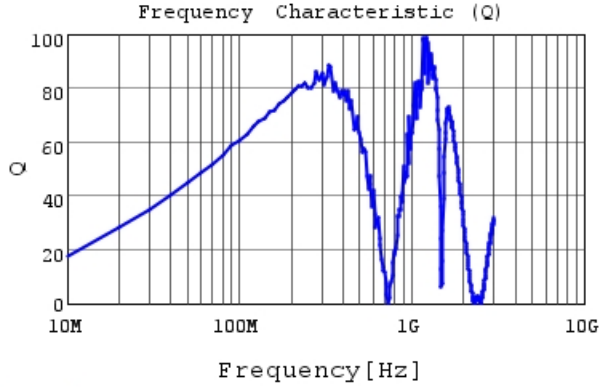
LQW2UASR27F00 Q
