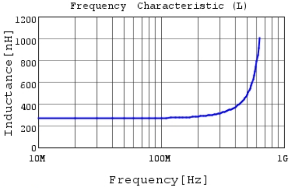
LQW2UASR27F00 L
