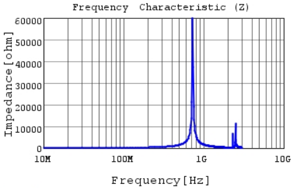
LQW2UASR27F00 |Z|
