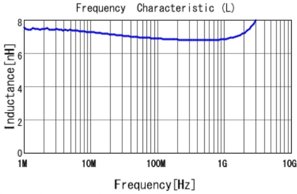
LQW18AN6N8G80 L
