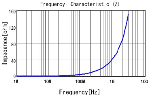
LQW18AN6N8G80 |Z|
