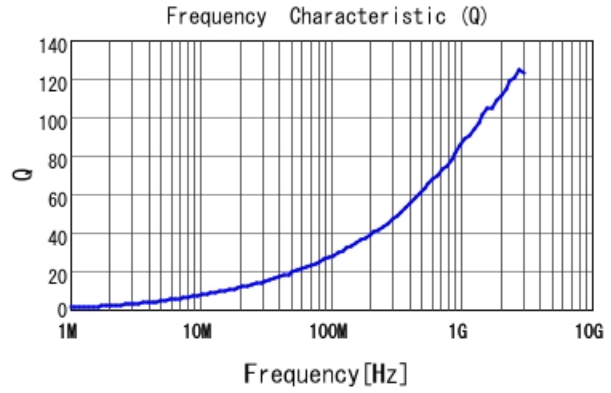
LQW18AN6N8G80 Q
