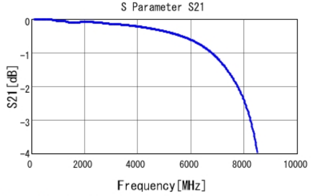
GRM1885C1H271GA01 S21 DCOV, 25degC
