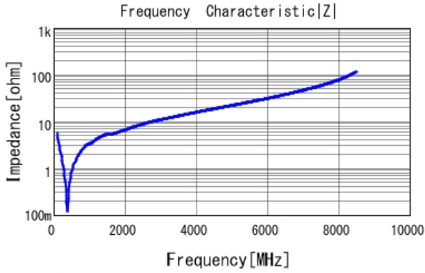
GRM1885C1H271GA01 |Z| DCOV, 25degC
