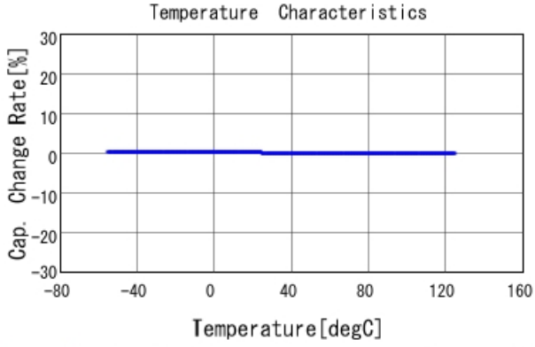
GRM1885C1H271GA01 C-Temp. capchange, DCOV, AC1Vrms
