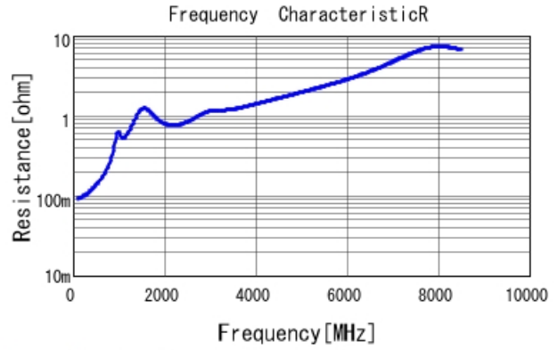
GRM1885C1H271GA01 R DCOV, 25degC
