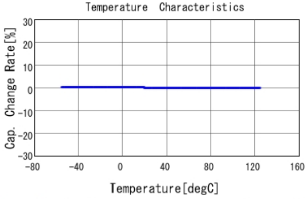
GRM2192C1H562JA01 C-Temp. capchange, DCOV, AC1Vrms
