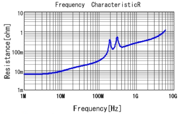
GRM2192C1H562JA01 R DCOV, 20degC
