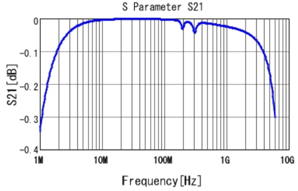
GRM2192C1H562JA01 S21 DCOV, 20degC
