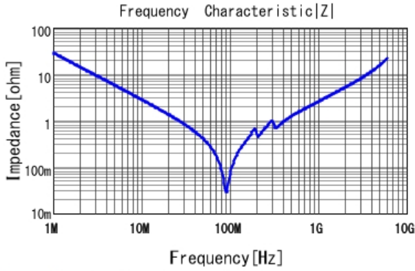
GRM2192C1H562JA01 |Z| DCOV, 20degC
