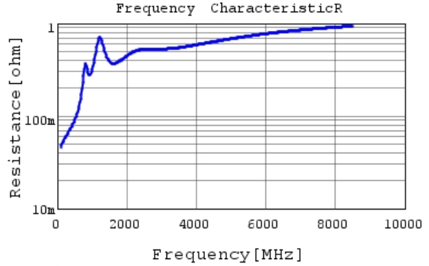
GCM1555C1H561FA16 R DC0V, 25degC
