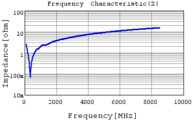
GCM1555C1H561FA16 |Z| DC0V, 25degC
