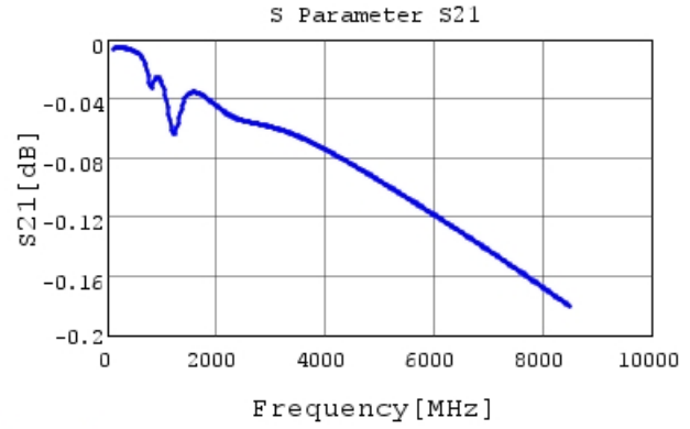
GCM1555C1H561FA16 S21 DCOV, 25degC
