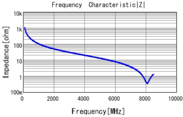
GJM0335C1E1R5CB01 |Z| DCOV, 25degC
