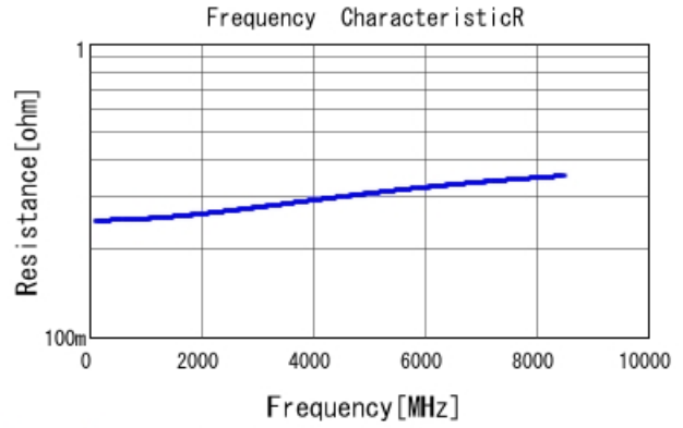
GJM0335C1E1R5CB01 R DCOV, 25degC
