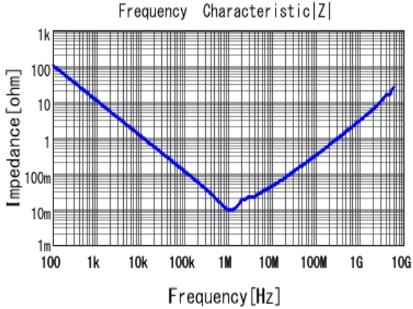
■ GRJ31CR70J226KE12 |Z| DCOV, 25degC
