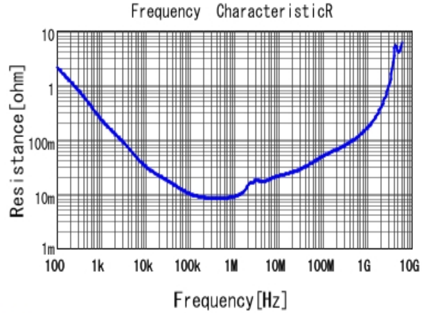
■ GRJ31CR70J226KE12 R DCOV, 25degC
