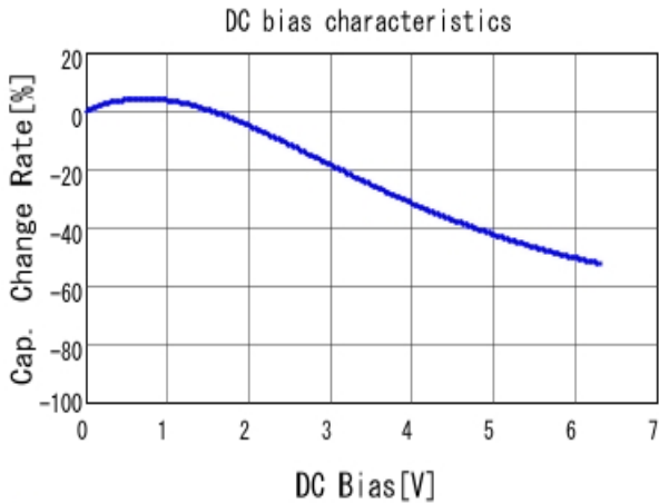
■ GRJ31CR70J226KE12 C-DC bias capchange, 25.0degC, AC0.
