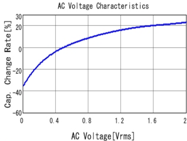
■ GRJ31CR70J226KE12 C-AC Voltage capchange, DCOV, 25.0d
