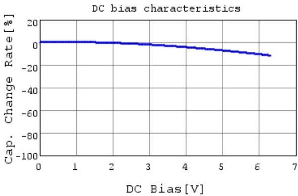
GRM033R60J103KA01 C-DC bias capchange, 25.0c
