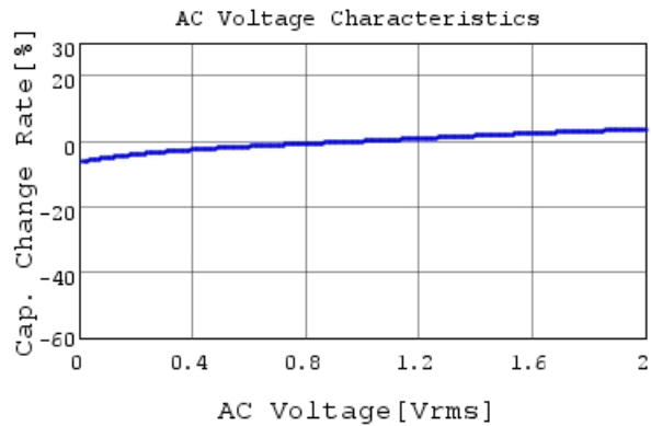
GRM033R60J103KA01 C-AC Voltage capchange, Dc
