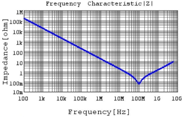
GRM033R60J103KA01 |Z| DCOV, 25degC
