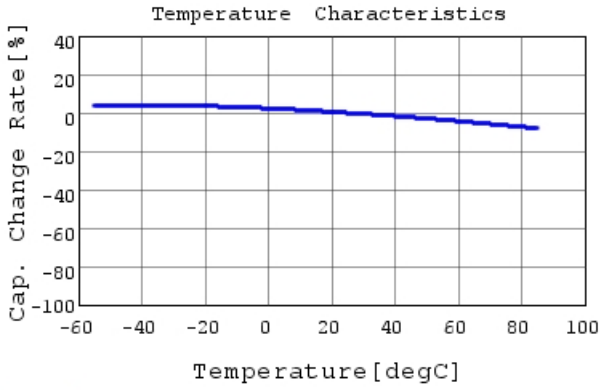
GRM033R60J103KA01 C-Temp. capchange, DC0.0V,
