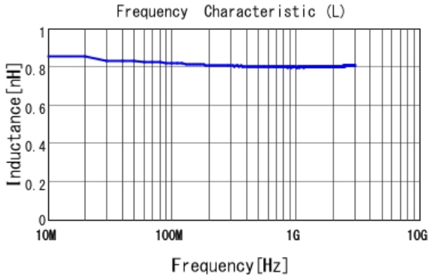
LQP03TN0N8B02 L
