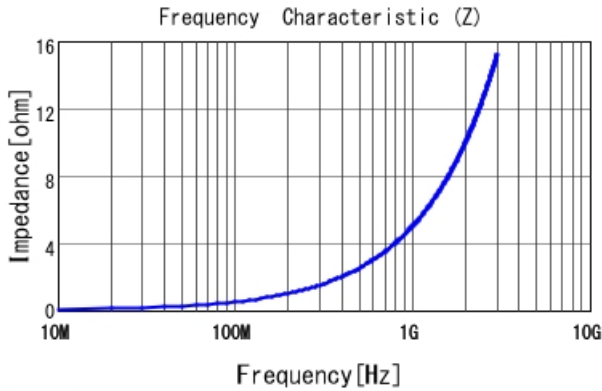
LQP03TN0N8B02 |Z|
