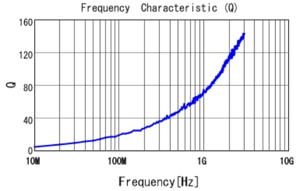
LQP03TN0N8B02 Q
