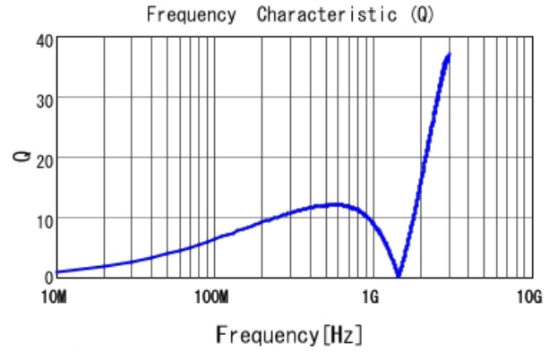
LQP03TN82NJ02 Q
