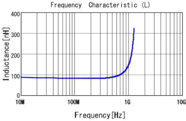
LQP03TN82NJ02 L
