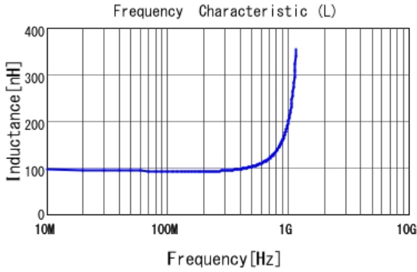
LQG15WZ91NJ02 L
