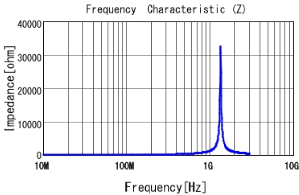
LQG15WZ91NJ02 |Z|
