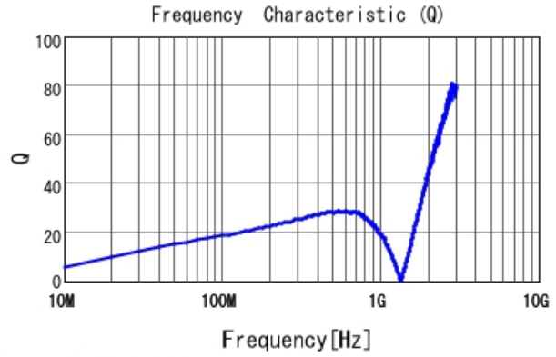
LQG15WZ91NJ02 Q
