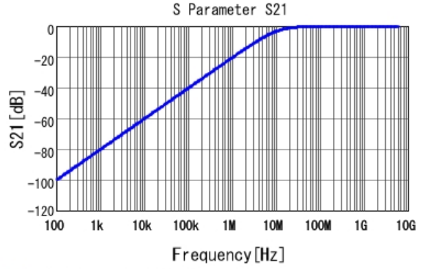
■ GRM033R71E151KA01 S21 DCOV, 25degC
