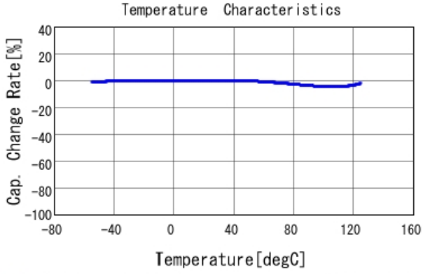
■ GRM033R71E151KA01 C-Temp. capchange, DCO. 0V, AC1. 0Vrm
