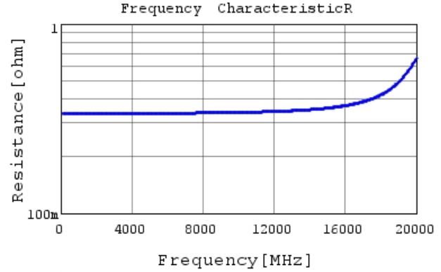
GJM0335C1E1R0CB01 R DCOV, 25degC
