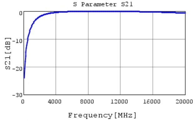
GJM0335C1E1R0CB01 S21 DCOV, 25degC
