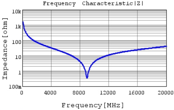
GJM0335C1E1R0CB01 |Z| DCOV, 25degC
