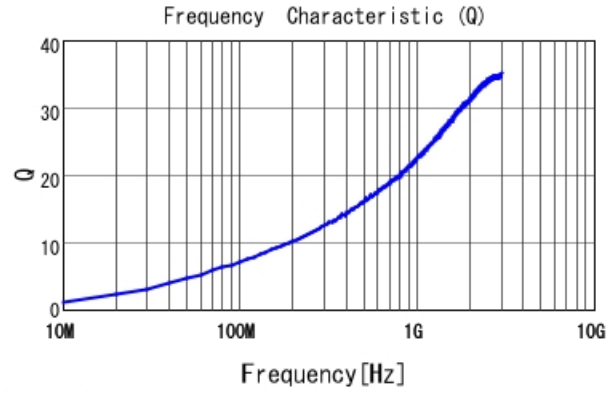
LQP03TG2N9C02 Q
