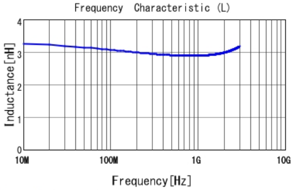
LQP03TG2N9C02 L
