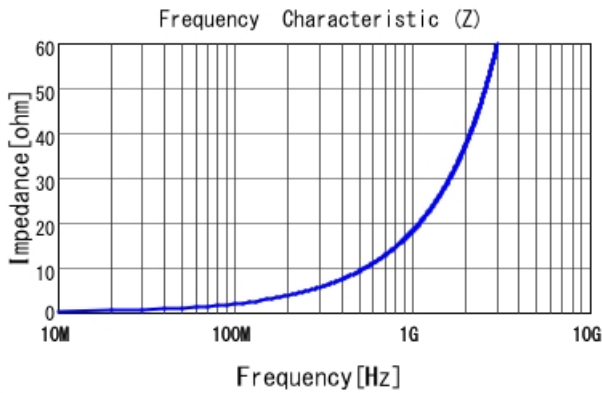
LQP03TG2N9C02 |Z|
