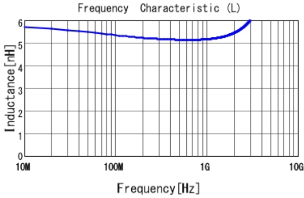
LQP03TQ5N1J02 L
