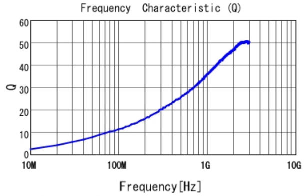
LQP03TQ5N1J02 Q
