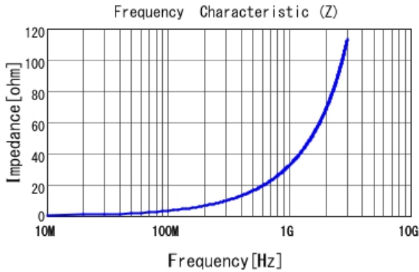
LQP03TQ5N1J02 |Z|
