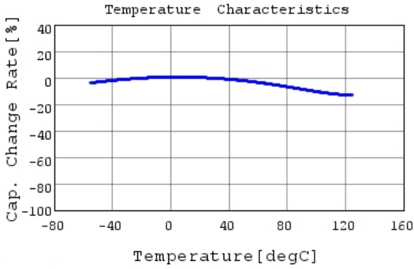
GRM155R70J473KA01 C-Temp. capchange, DC0.0V,
