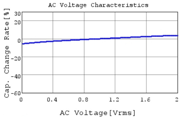
GRM155R70J473KA01 C-AC Voltage capchange, DC
