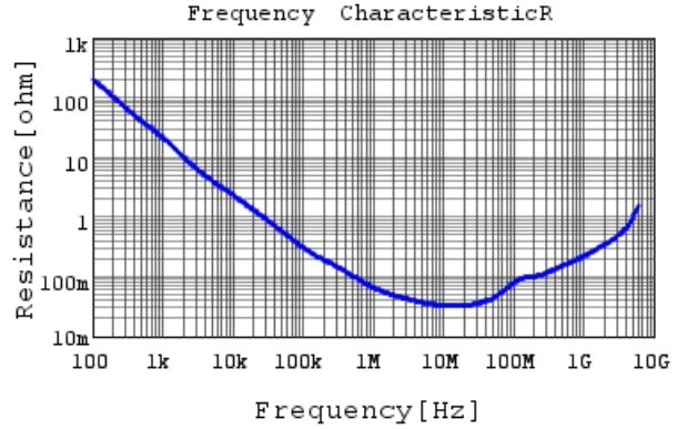
GRM155R70J473KA01 R DC0V, 25degC
