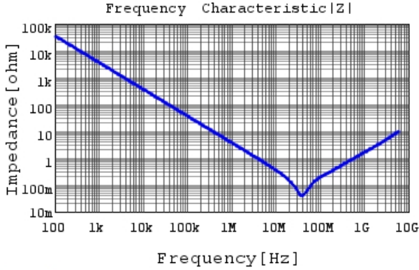
GRM155R70J473KA01 |Z| DC0V, 25degC
