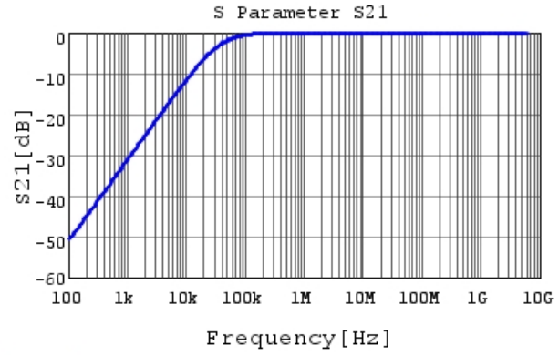
GRM155R70J473KA01 S21 DC0V, 25degC
