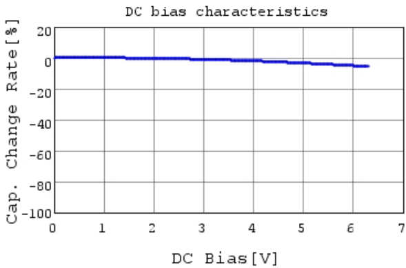
GRM155R70J473KA01 C-DC bias capchange, 25.0c
