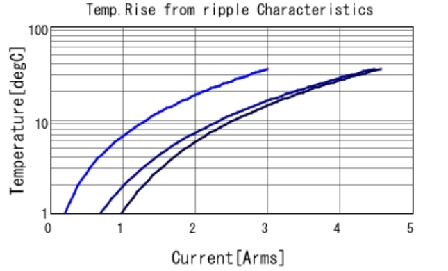
GRM188R61A475KE15 Temp. rise — 100kHz — 500
