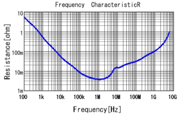
GRM188R61A475KE15 R DCOV, 25degC
