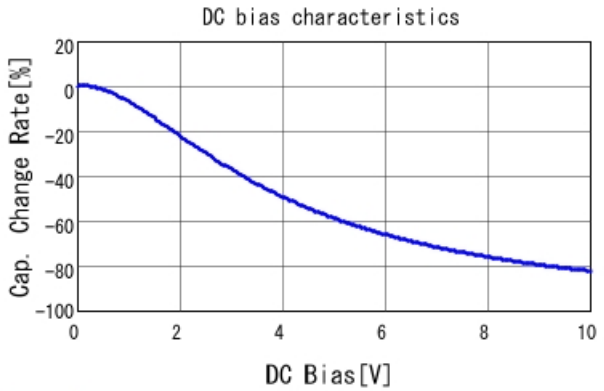
GRM188R61A475KE15 C-DC bias capchange, 25.0degC, A
