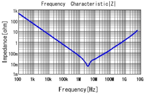
GRM188R61A475KE15 |Z| DCOV, 25degC
