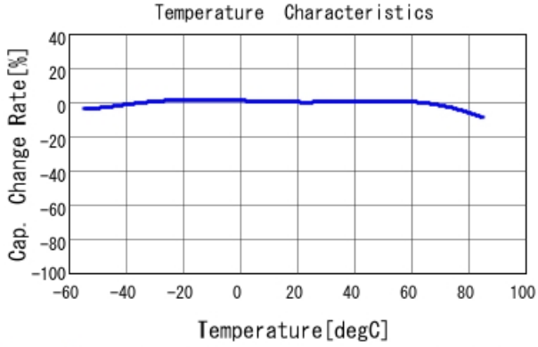
GRM188R61A475KE15 C-Temp. capchange, DC0.0V, AC0.5
