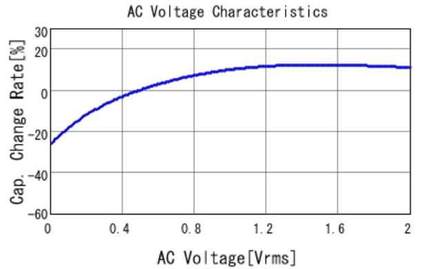
GRM188R61A475KE15 C-AC Voltage capchange, DCOV, 25
