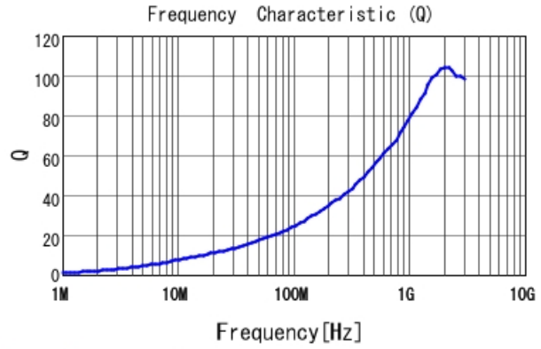
LQW15AN6N2G80 Q
