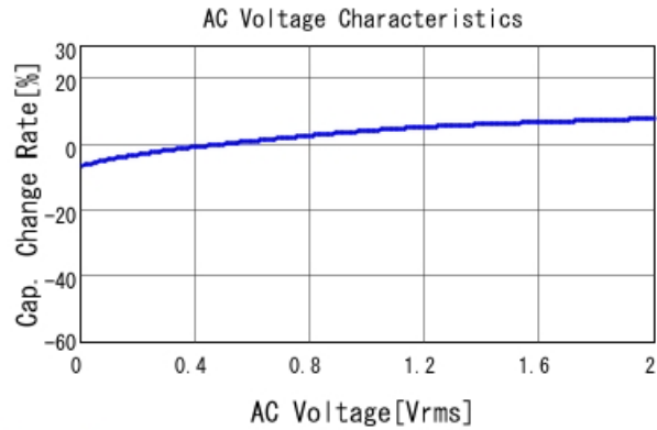
GRM152R60J104ME19 C-AC Voltage capchange, DCOV, 25
