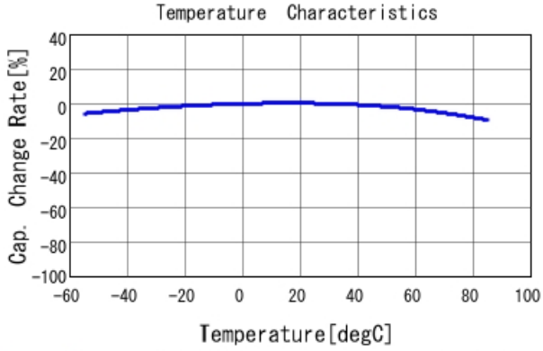
GRM152R60J104ME19 C-Temp. capchange, DC0.0V, AC0.5
