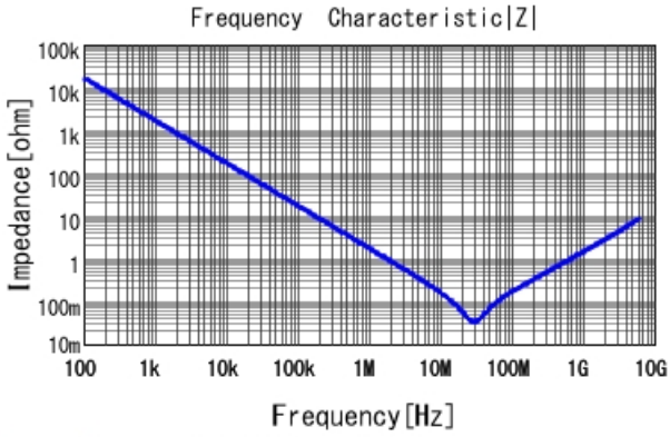
GRM152R60J104ME19 |Z| DCOV, 25degC
