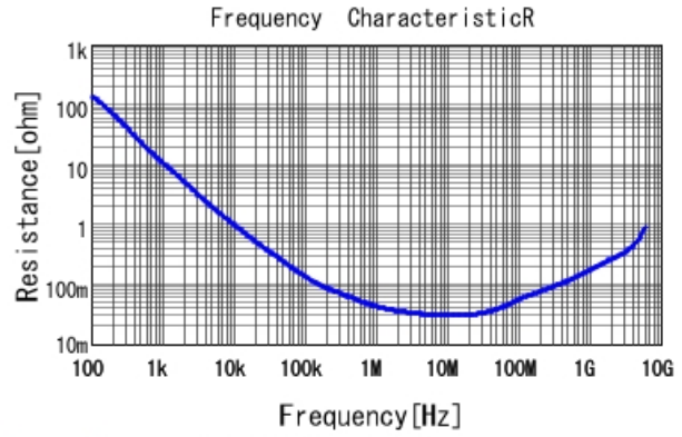
GRM152R60J104ME19 R DCOV, 25degC
