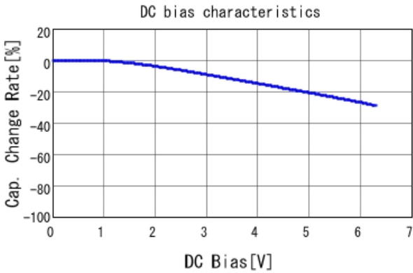
GRM152R60J104ME19 C-DC bias capchange, 25.0degC, A
