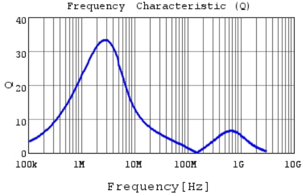
LQH2HPZ1R5MDR Q
