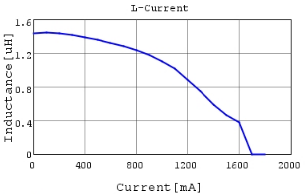
LQH2HPZ1R5MDR L-Current 20degC
