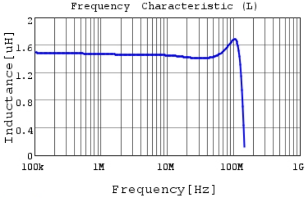
LQH2HPZ1R5MDR L
