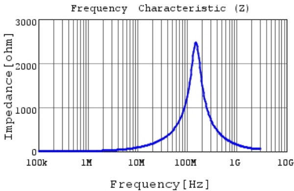
LQH2HPZ1R5MDR |Z|
