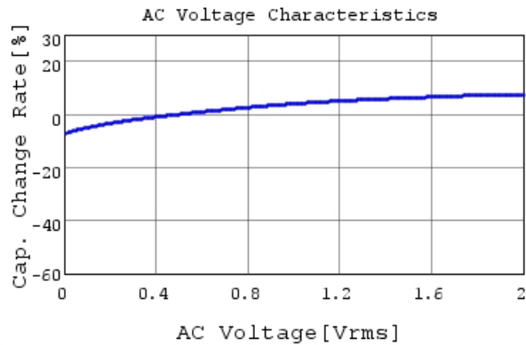
GRM033R60J223KE01 C-AC Voltage capchange, Dc
