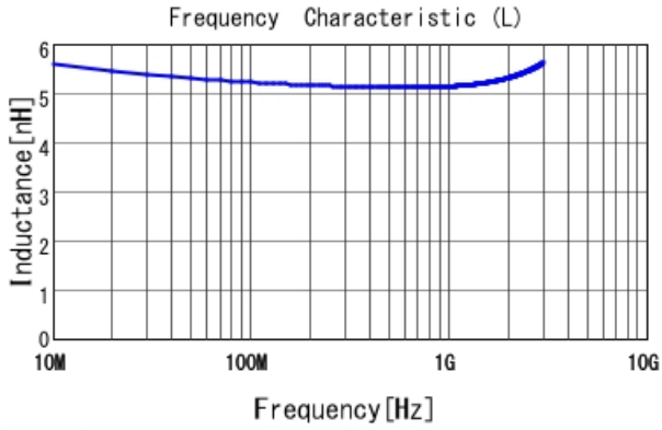
LQW15AN5N1D10 L
