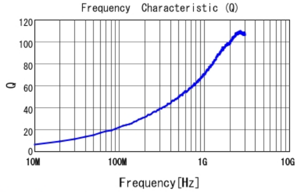
LQW15AN5N1D10 Q
