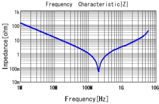
GRM2165C1H122JA01 |Z| DCOV, 25degC
