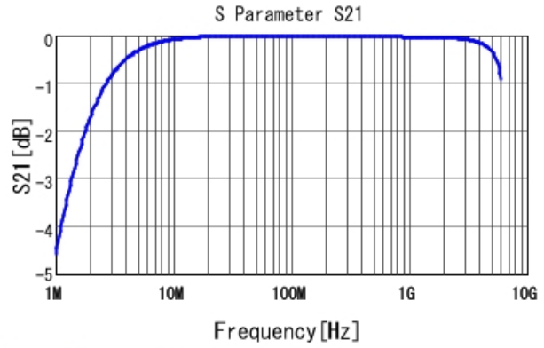
GRM2165C1H122JA01 S21 DCOV, 25degC
