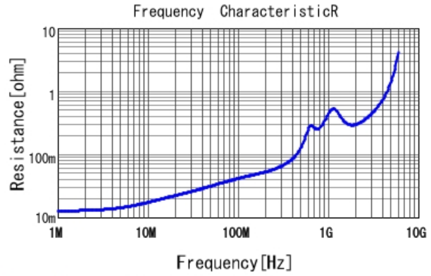
GRM2165C1H122JA01 R DCOV, 25degC
