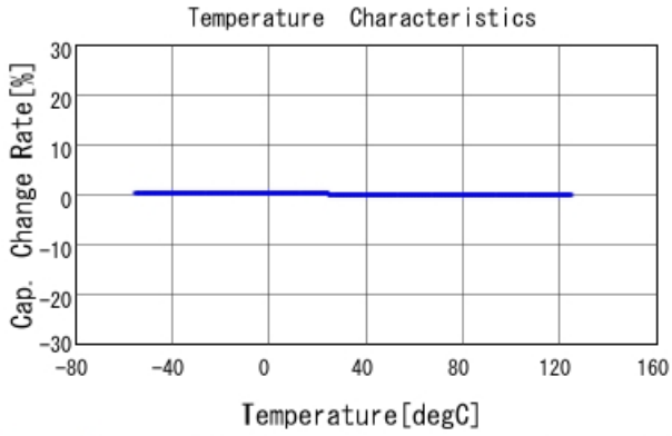
GRM2165C1H122JA01 C-Temp. capchange, DCOV, AC1Vrms
