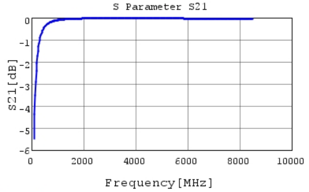
GRM0225C1H100JA03 S21 DCOV, 25degC
