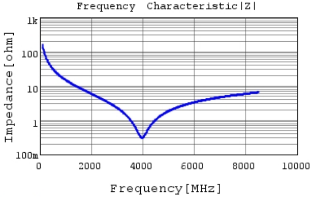
GRM0225C1H100JA03 |Z| DCOV, 25degC
