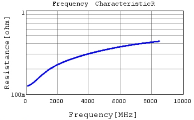
GRM0225C1H100JA03 R DCOV, 25degC
