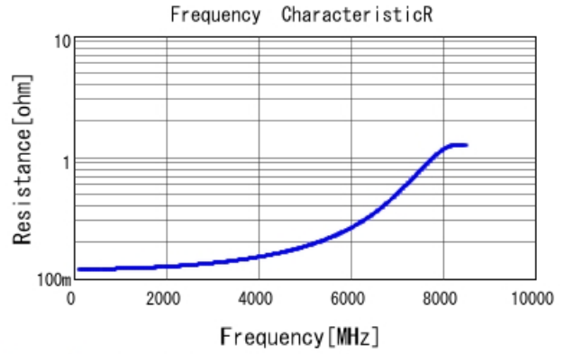
GQM1875C2E3R3BB12 R DCOV, 25degC
