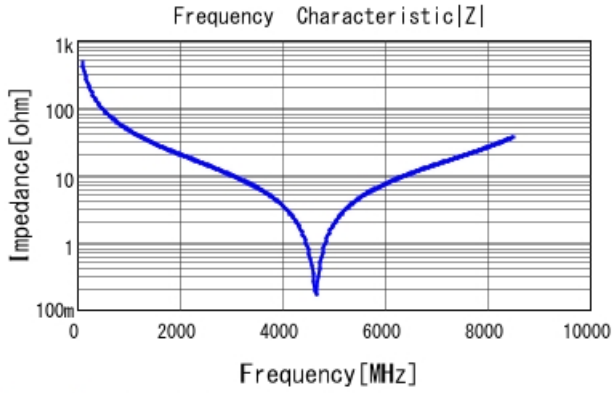
GQM1875C2E3R3BB12 |Z| DCOV, 25degC
