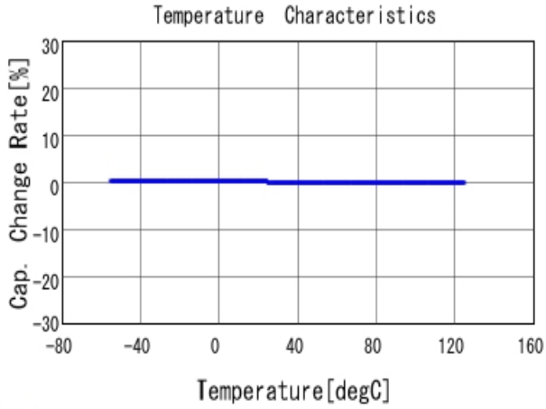
■ GRM1555C1H121JA01 C-Temp. capchange, DCOV, AC1Vrms
