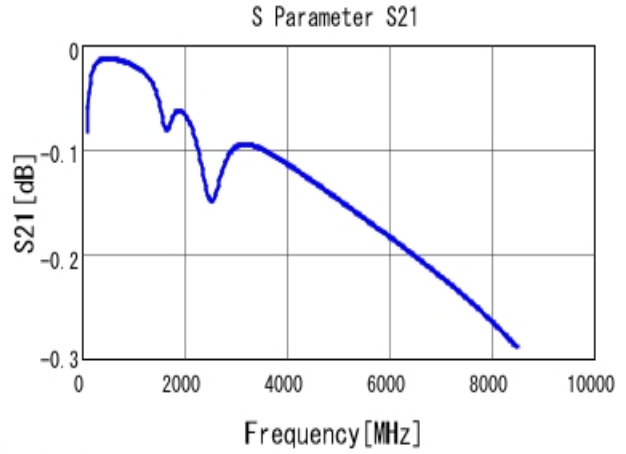
■ GRM1555C1H121JA01 S21 DCOV, 25degC
