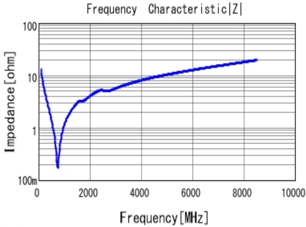
■ GRM1555C1H121JA01 |Z| DCOV, 25degC
