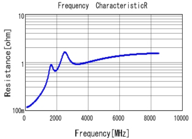
■ GRM1555C1H121JA01 R DCOV, 25degC
