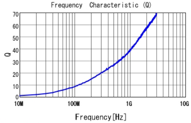
LQP15MN1N5W02 Q
