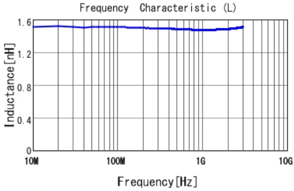
LQP15MN1N5W02 L
