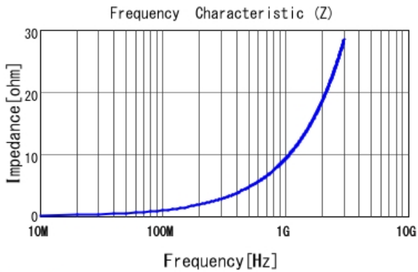
LQP15MN1N5W02 |Z|
