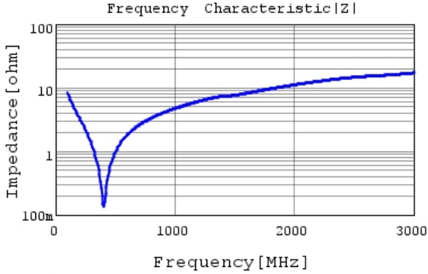
GRM31A5C2J181JW01 |Z| DCOV, 25degC
