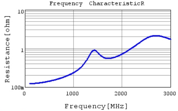
GRM31A5C2J181JW01 R DCOV, 25degC
