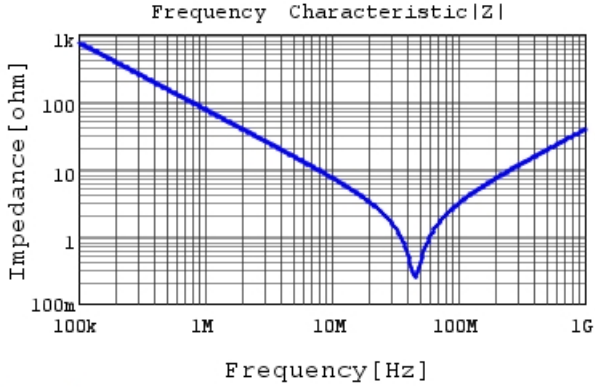
RDER71H222K0K1H03B |Z| DCOV, 25degC
