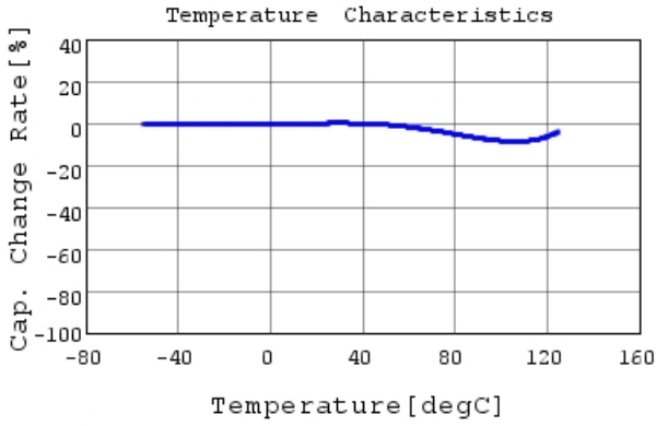
■ RDER71H222K0K1H03B C-Temp. capchange, DC0.0V
