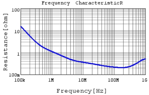
RDER71H222K0K1H03B R DCOV, 25degC
