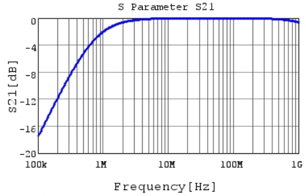
■ RDER71H222K0K1H03B S21 DC0V, 25degC
