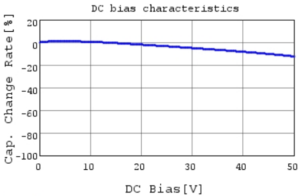
RDER71H222K0K1H03B C-DC bias capchange, 25.0
