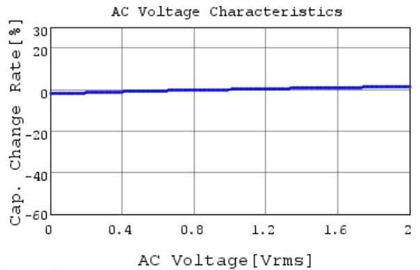
RDER71H222K0K1H03B C-AC Voltage capchange, I
