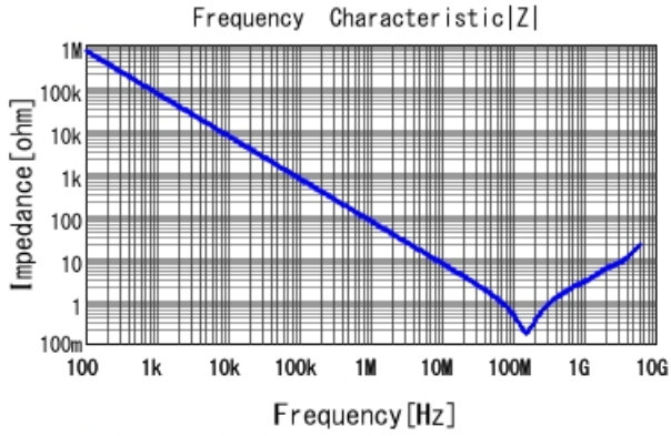
GRJ216R71H222KE01 |Z| DCOV, 25degC
