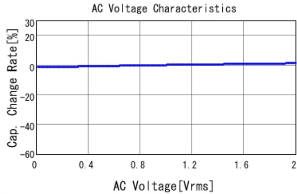
GRJ216R71H222KE01 C-AC Voltage capchange, DCOV, 25
