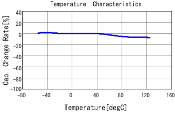
GRJ216R71H222KE01 C-Temp. capchange, DC0.0V, AC1.C
