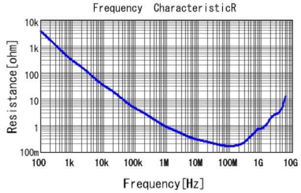
GRJ216R71H222KE01 R DCOV, 25degC
