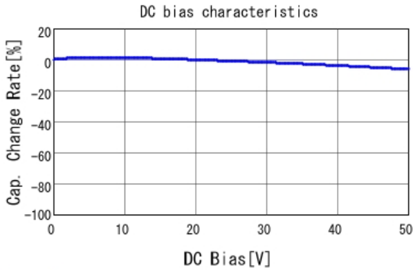
GRJ216R71H222KE01 C-DC bias capchange, 25.0degC, A
