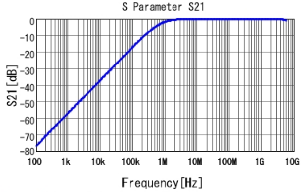
GRJ216R71H222KE01 S21 DC0V, 25degC
