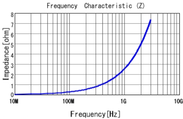
LQP02HQ0N4B02 |Z|
