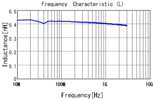
LQP02HQ0N4B02 L
