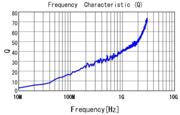
LQP02HQ0N4B02 Q
