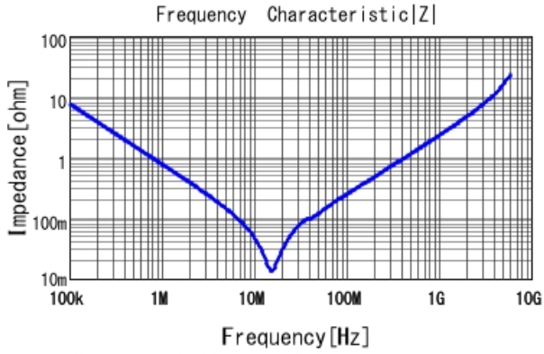
GRM188B11A224KA01 |Z| DCOV, 20degC
