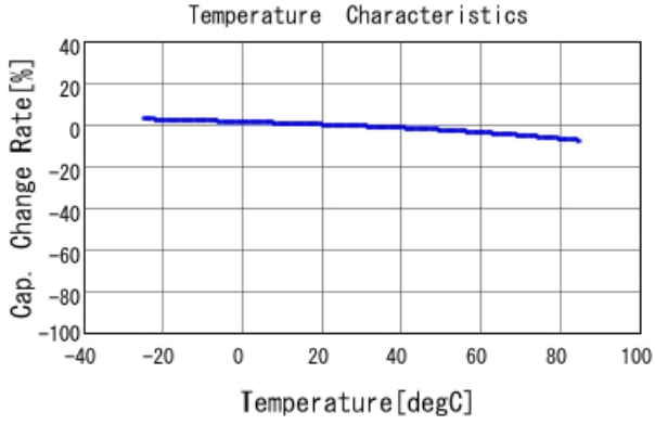
GRM188B11A224KA01 C-Temp. capchange, DC0.0V, AC1.C
