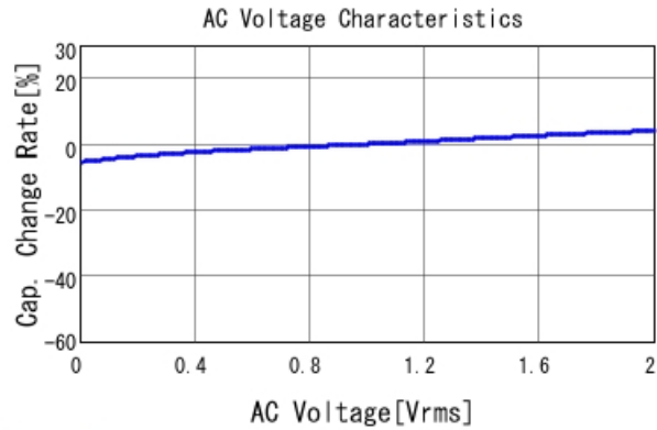
GRM188B11A224KA01 C-AC Voltage capchange, DCOV, 2C
