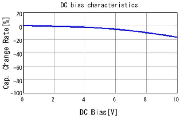
GRM188B11A224KA01 C-DC bias capchange, 20.0degC, A
