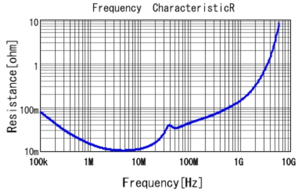
GRM188B11A224KA01 R DCOV, 20degC
