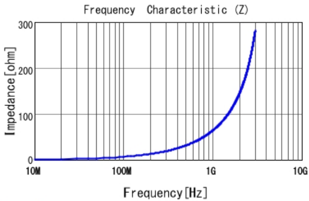
LQP03TN10NHZ2 |Z|
