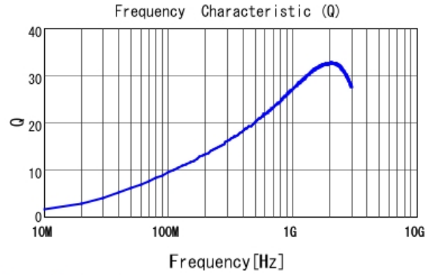
LQP03TN10NHZ2 Q
