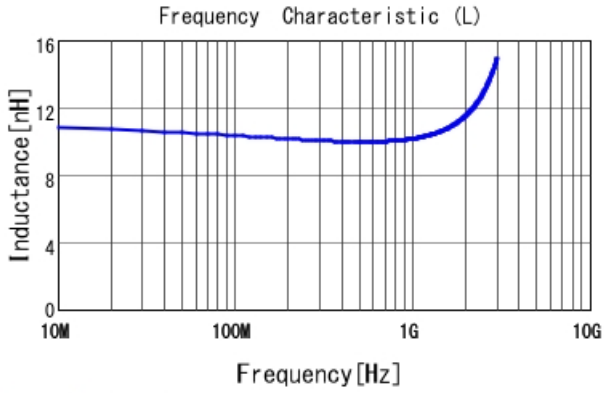
LQP03TN10NHZ2 L
