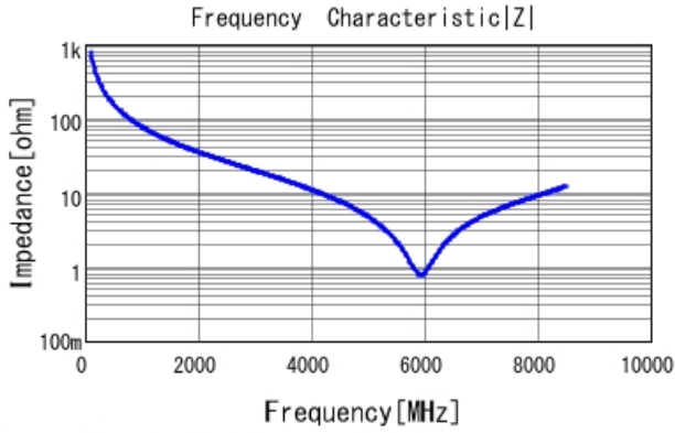
GRM1555C1H2R0WA01 |Z| DCOV, 25degC
