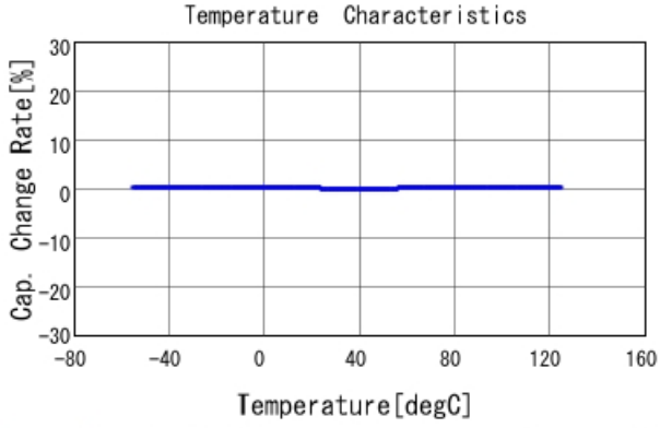
GRM1555C1H2R0WA01 C-Temp. capchange, DCOV, AC1Vrms
