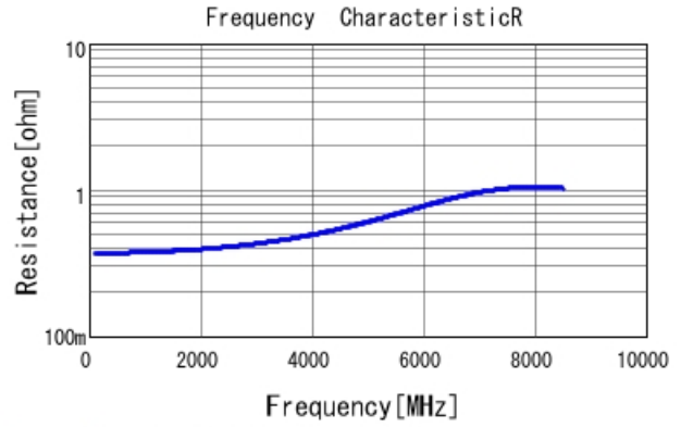
GRM1555C1H2R0WA01 R DCOV, 25degC
