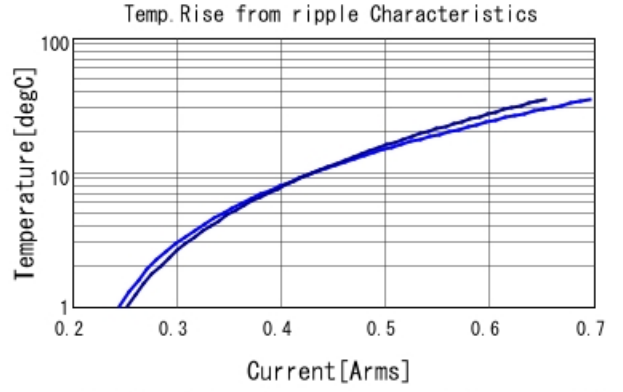
GRM1555C1H2R0WA01 Temp. rise — 2GHz — 3GHz
