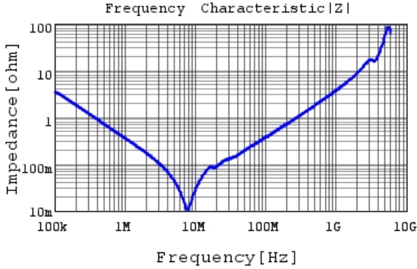
GRM43DR72E474KW01 |Z| DCOV, 25degC
