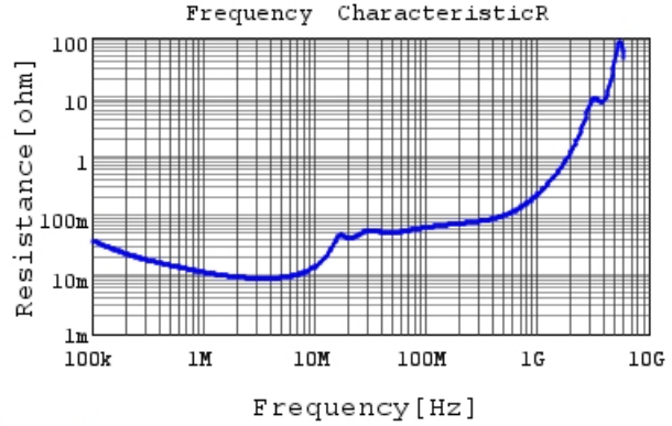
GRM43DR72E474KW01 R DCOV, 25degC
