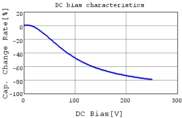
GRM43DR72E474KW01 C-DC bias capchange, 25.0c
