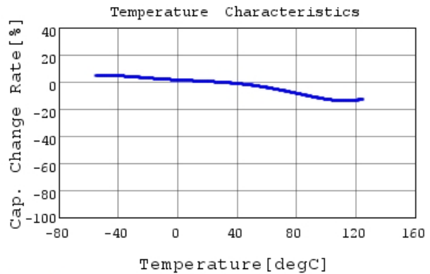
GRM43DR72E474KW01 C-Temp. capchange, DCOV, 1
