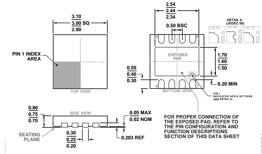
Figure 71. 8-Lead Lead Frame Chip Scale Package [LFCSP] 3 mm x 3 mm Body and 0.75 mm Package Height (CP-8-21) Dimensions shown in millimeters
