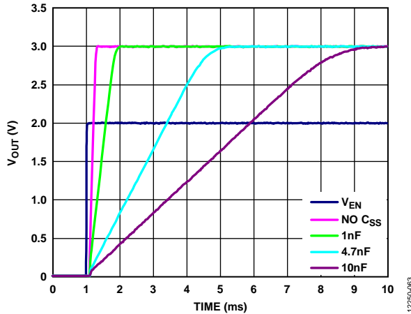
Figure 62. Typical Soft Start Behavior, Different C SS Values
