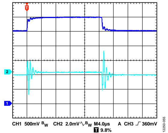
Figure 54. Line Transient Response, 2.5 V to 3 V, I_{LOAD} = 2 A , Adjustable Version, V_{OUT} = 1.2 V , CH1 = V_{IN} , CH2 = V_{OUT}
