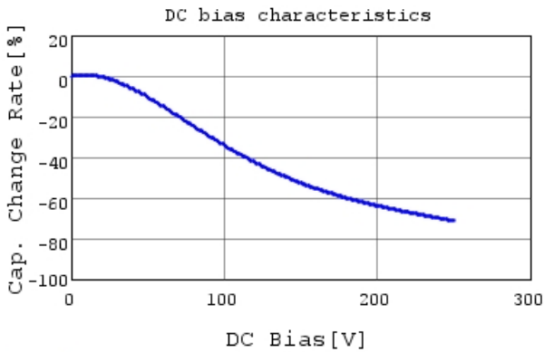
GRM55DR72E474KW01 C-DC bias capchange, 25.0c
