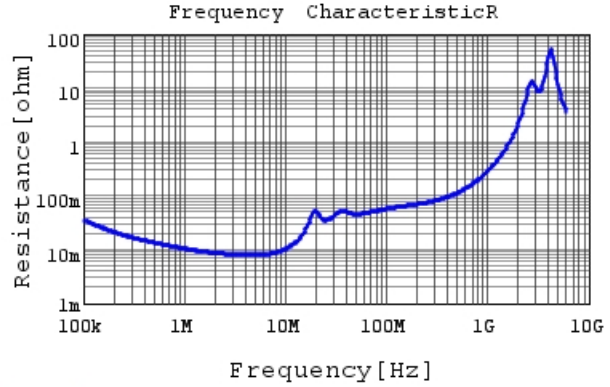
GRM55DR72E474KW01 R DCOV, 25degC
