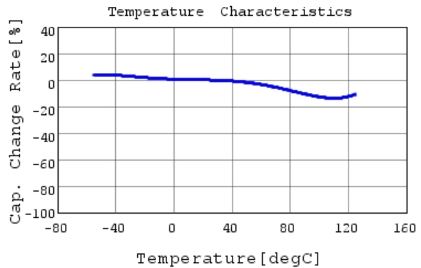
GRM55DR72E474KW01 C-Temp. capchange, DCOV, 1
