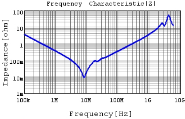
GRM55DR72E474KW01 |Z| DCOV, 25degC
