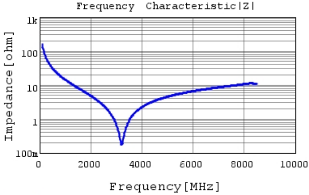
GJM0335C1E100JB01 |Z| DCOV, 25degC
