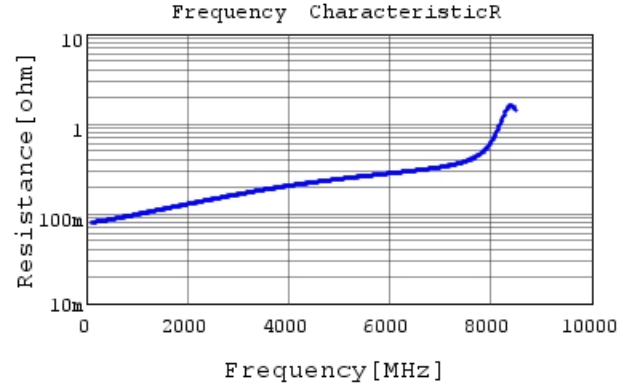
GJM0335C1E100JB01 R DCOV, 25degC
