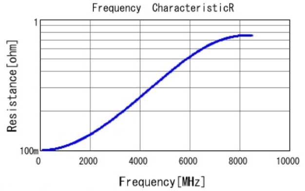
GJM0335C1E7R5CB01 R DCOV, 25degC
