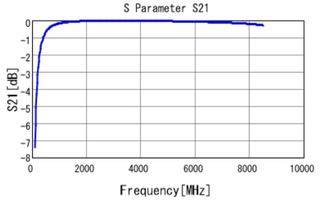
GJM0335C1E7R5CB01 S21 DC0V, 25degC
