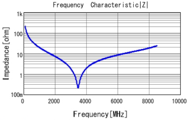
GJM0335C1E7R5CB01 |Z| DCOV, 25degC
