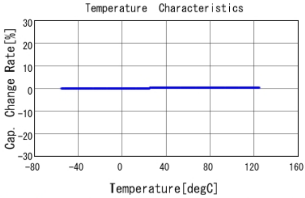
GJM0335C1E7R5CB01 C-Temp. capchange, DC0V, AC1Vrms
