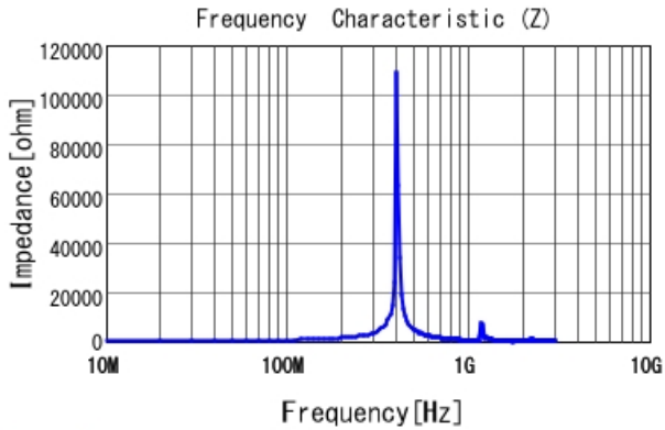
LQW2UASR91F00 |Z|
