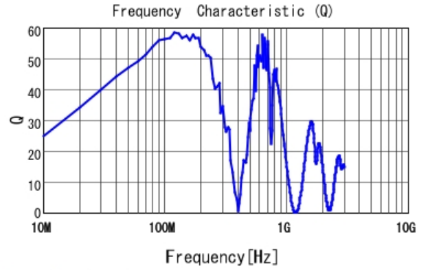
LQW2UASR91F00 Q
