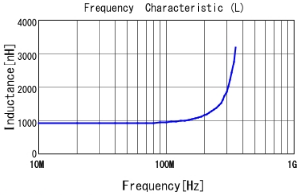
LQW2UASR91F00 L
