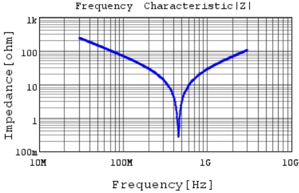
RDE5C1H220J0S1H03A |Z| DCOV, 25degC
