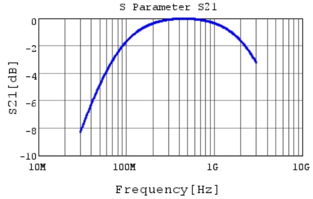
RDE5C1H220J0S1H03A S21 DCOV, 25degC
