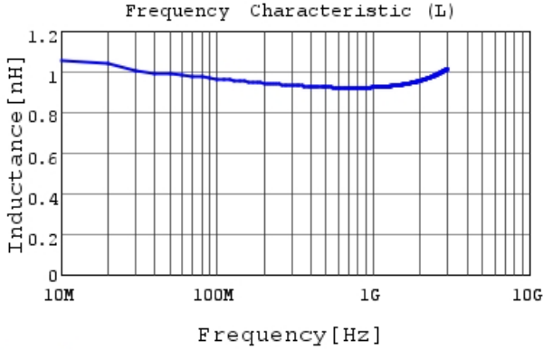
LQG15HS1N0B02 L
