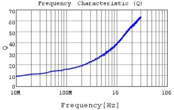
LQG15HS1N0B02 Q
