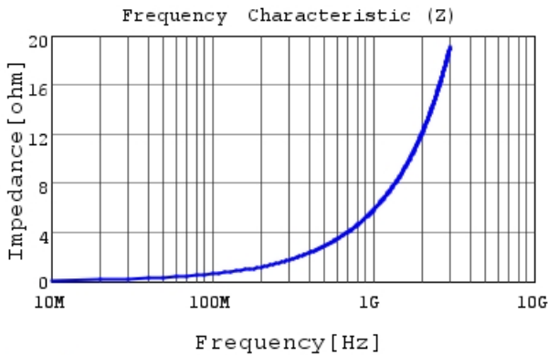
LQG15HS1N0B02 |Z|
