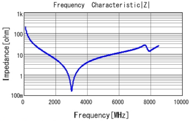
GJM1555C1H8R2WB01 |Z| DCOV, 25degC
