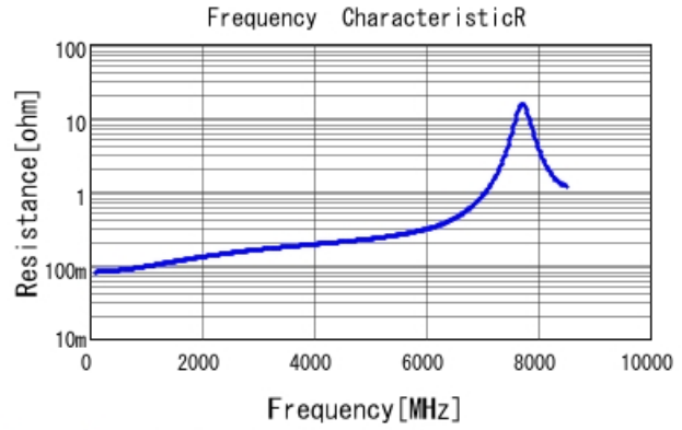
GJM1555C1H8R2WB01 R DCOV, 25degC
