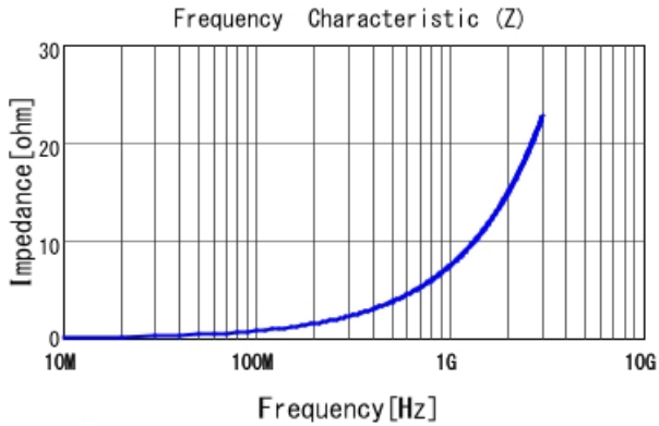
LQP15MN1N2B02 |Z|
