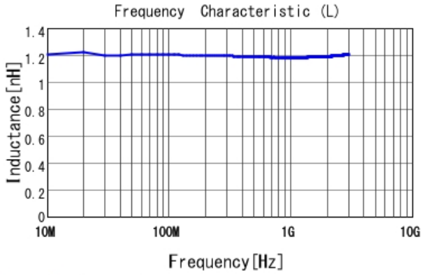
LQP15MN1N2B02 L
