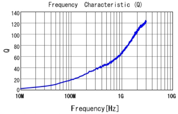
LQP15MN1N2B02 Q
