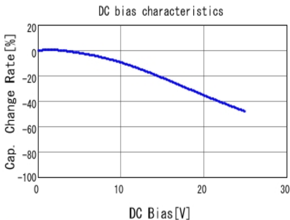
■ GRM155R71E333KA88 C-DC bias capchange, 25.0degC, AC1.
