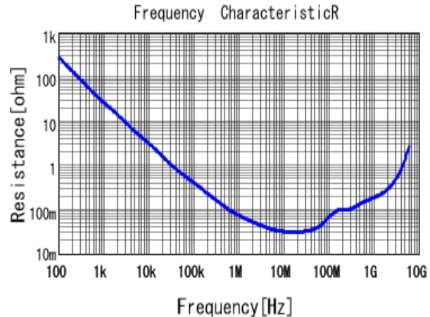
■ GRM155R71E333KA88 R DC0V, 25degC
