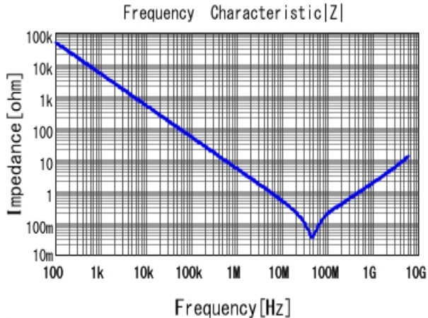
■ GRM155R71E333KA88 |Z| DC0V, 25degC
