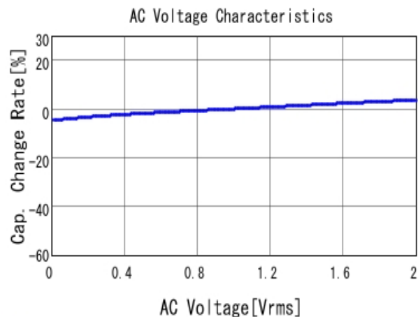
■ GRM155R71E333KA88 C-AC Voltage capchange, DC0V, 25.0d
